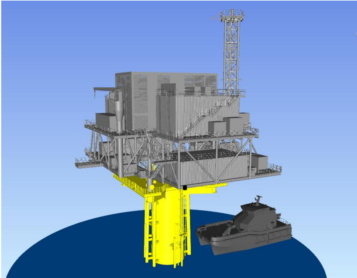
Figure 4.9: OSP topside general arrangement
