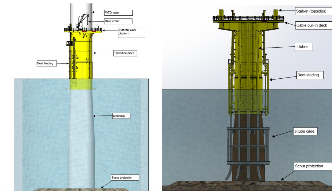
Figure 4.10: Typical monopile foundation general arrangement (left WTG, right OSP)
