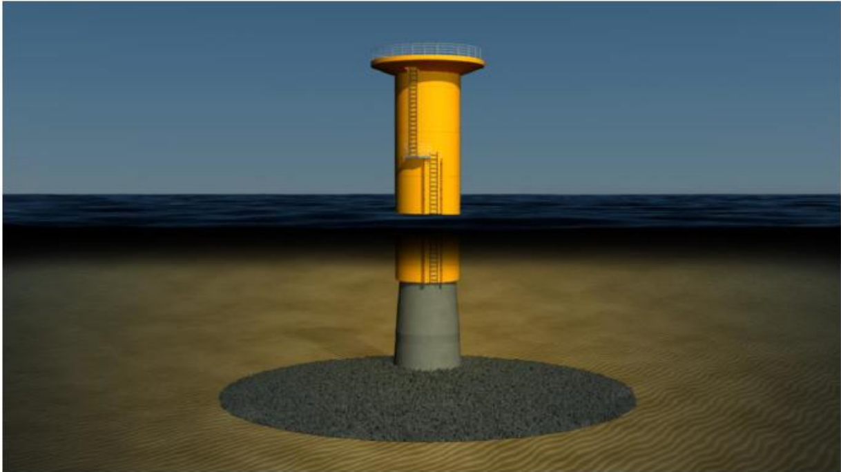
Figure 4.11: Image showing Scour protection (Rock) installed around monopile (Image courtesy of Dogger Bank Windfarm)
