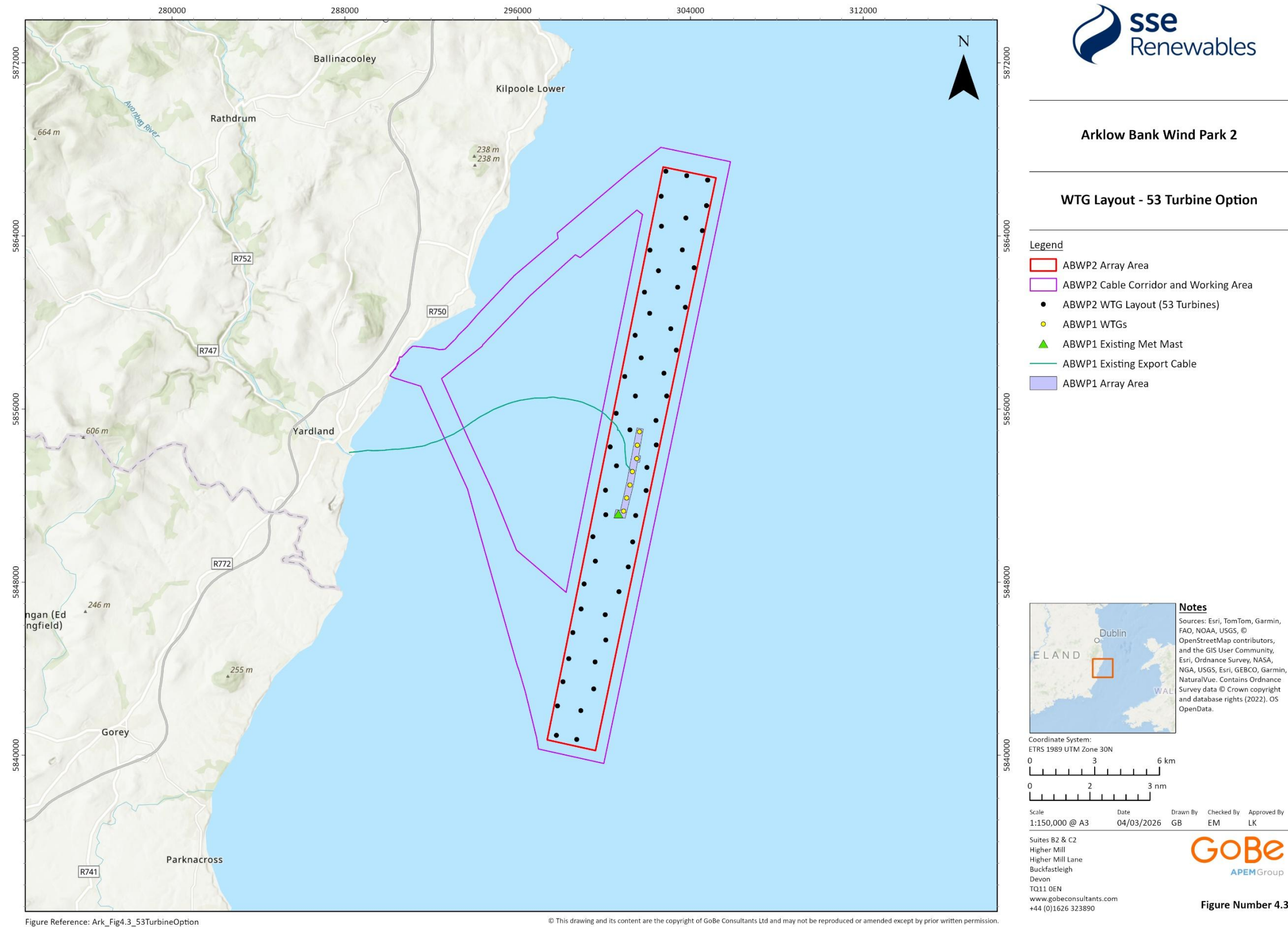
Figure 4.3: Proposed Development Project Design Option 1 (53 WTGs)
