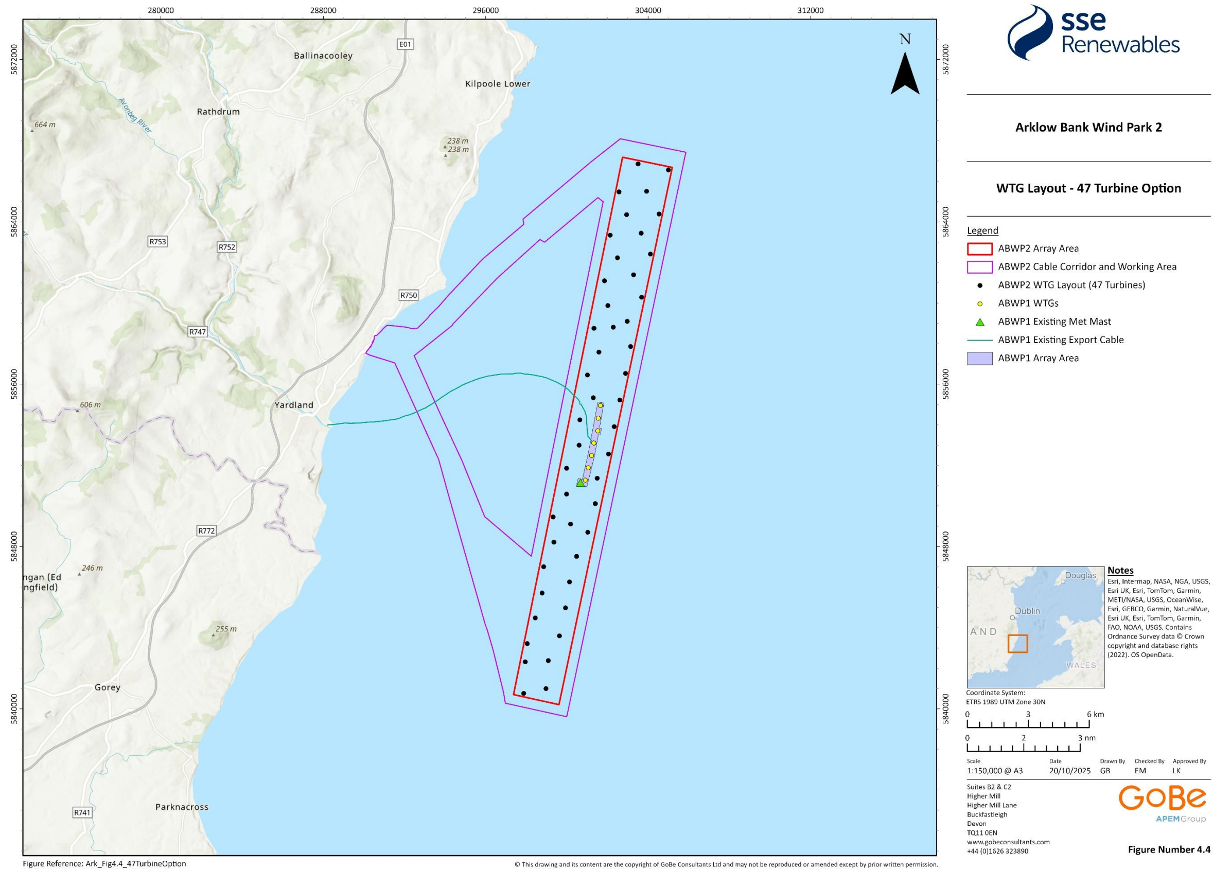
Figure 4.4: Proposed Development Project Design Option 2 (47 WTGs)
