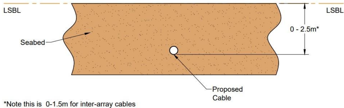
Figure 4.13: Example figure of proposed cable buried under LSBL
