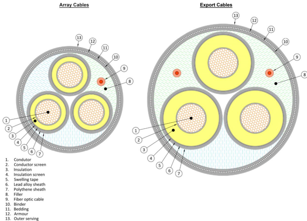
Figure 4.12: Example of submarine cable cross section
